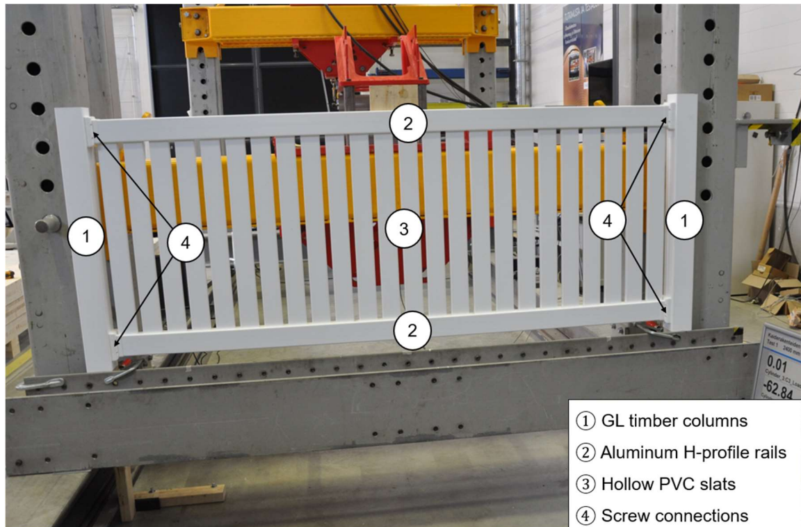
Figure 2. Assembled fence structure before the test.
