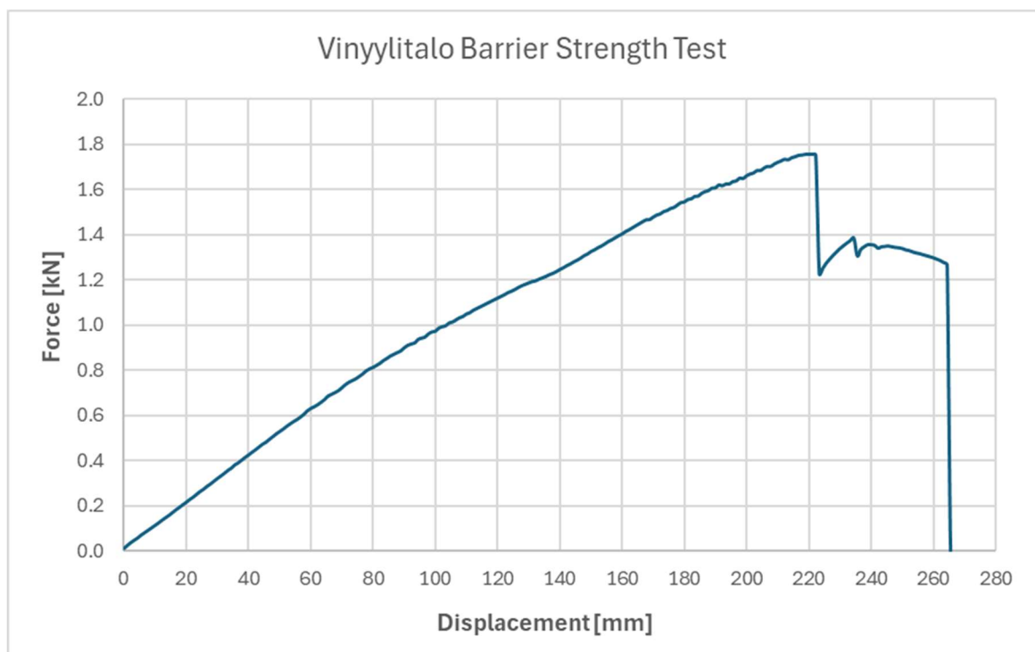
Figure 4. Force versus displacement curve of the test.
