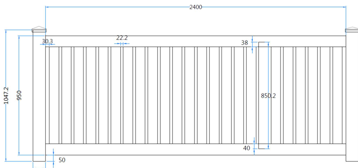
Figure 1. Dimensional drawing of the tested structure.
