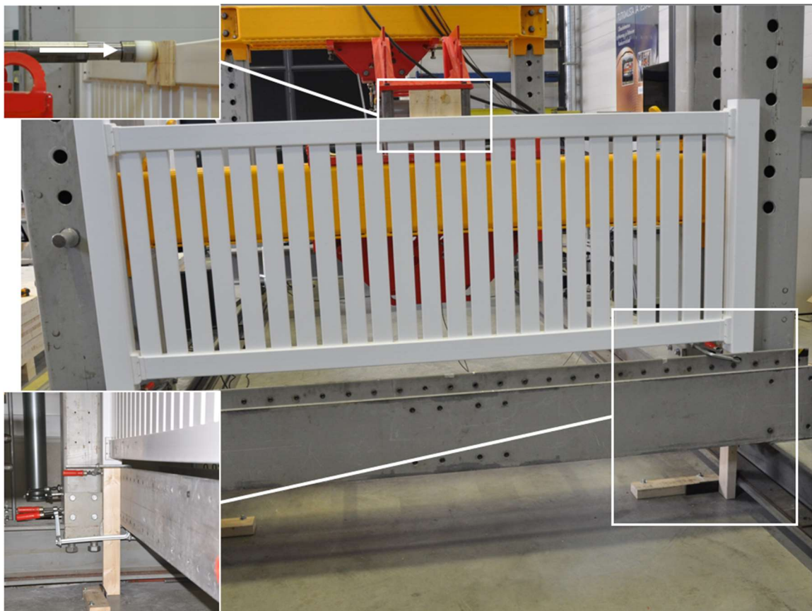
Figure 3. Barrier strength test arrangement.
